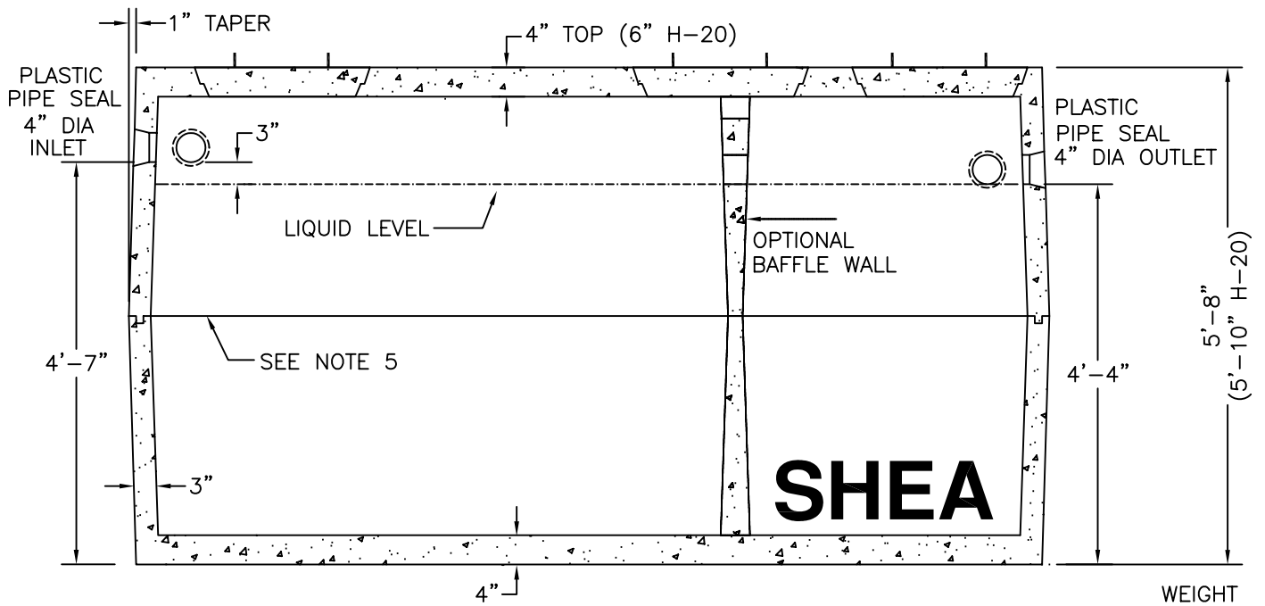
SECTION VIEW
