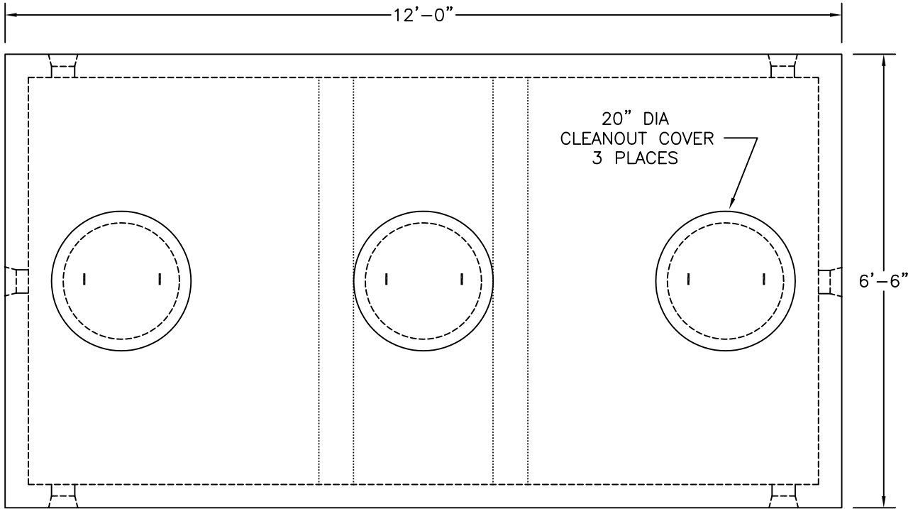
PLAN VIEW
