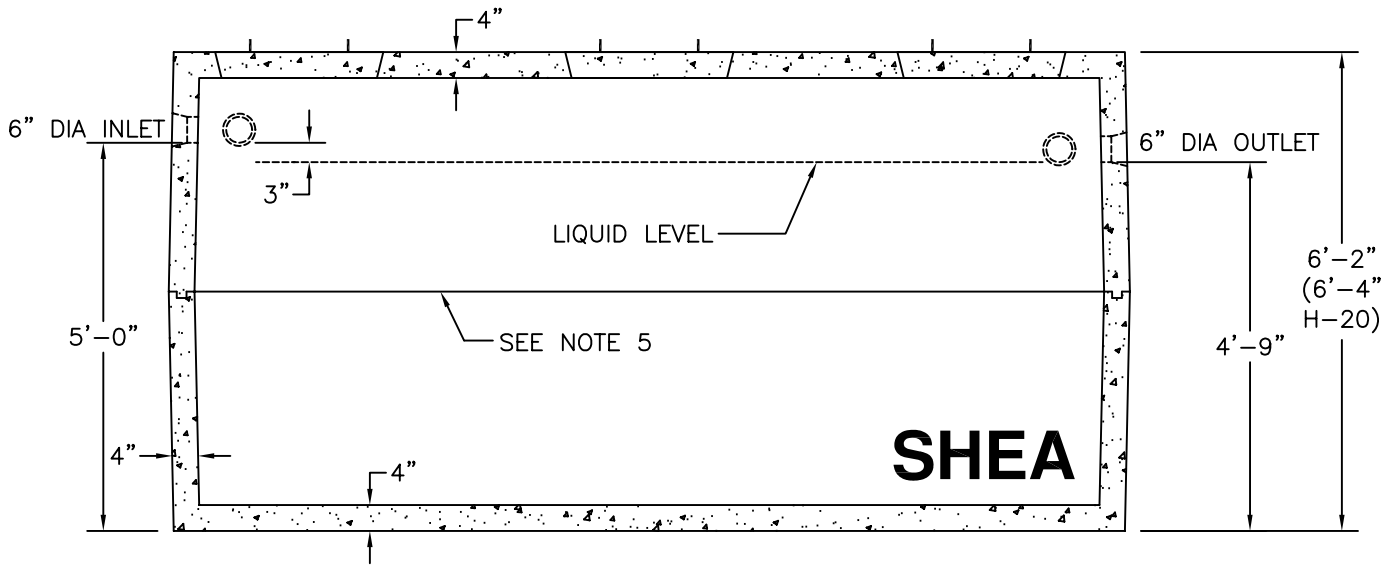
SECTION VIEW
