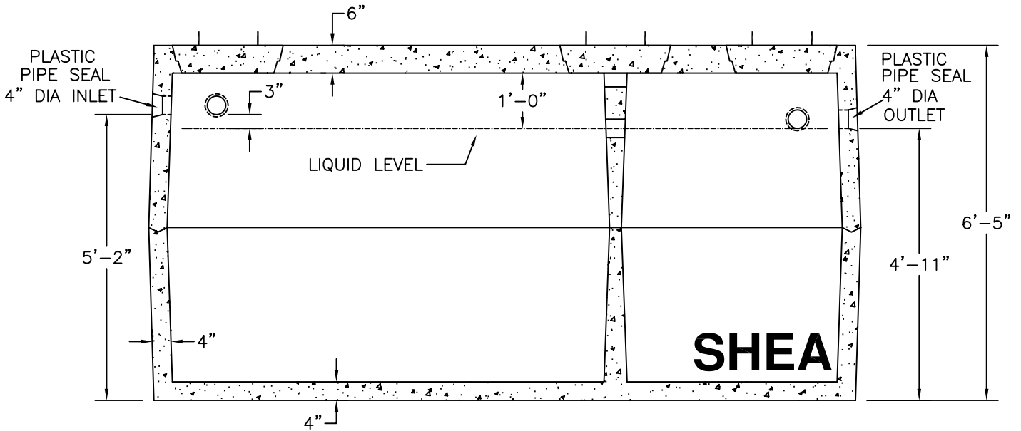
SECTION VIEW
