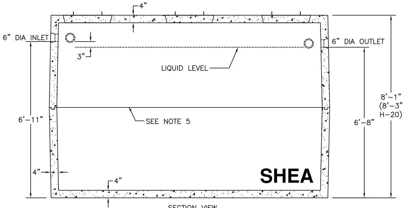
SECTION VIEW
