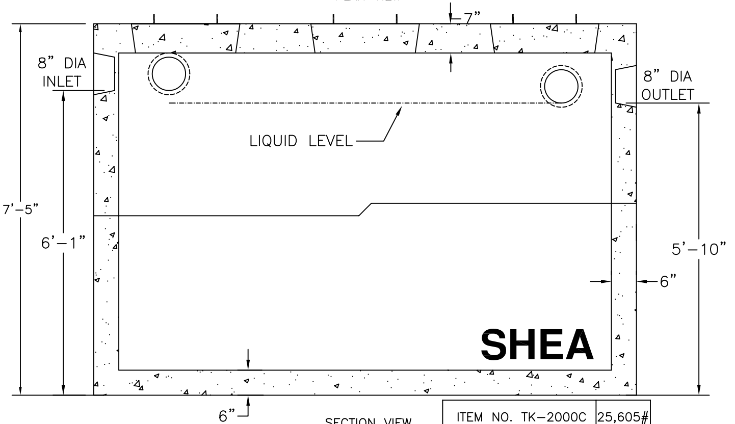
SECTION VIEW
