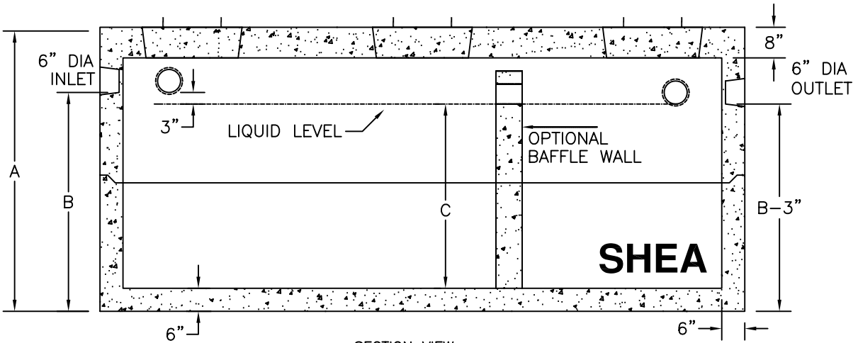
SECTION VIEW
