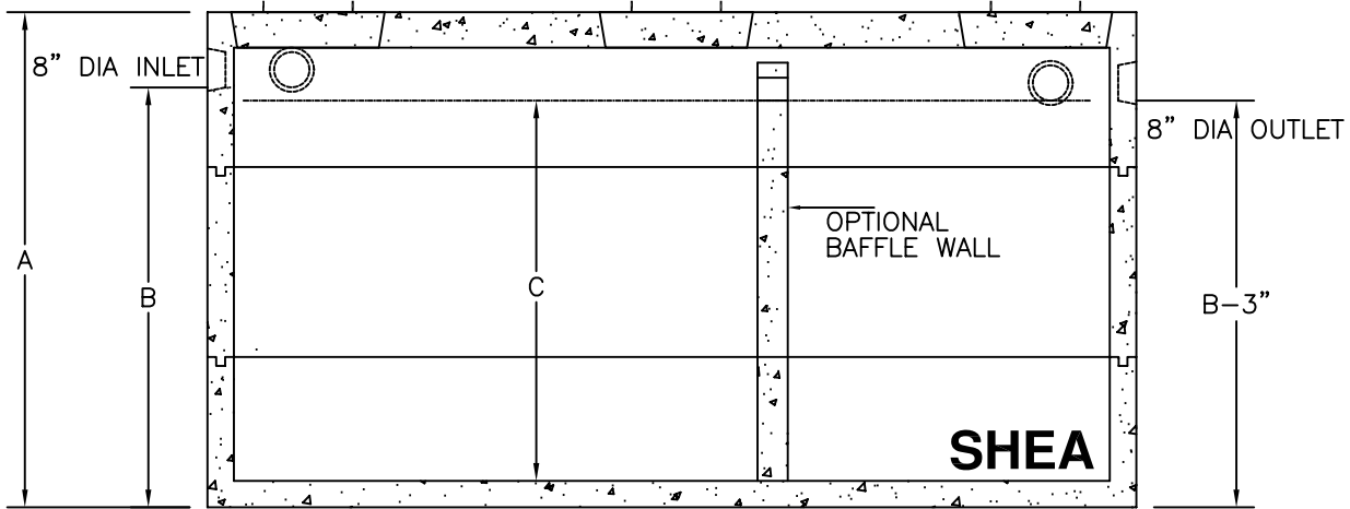
SECTION VIEW
