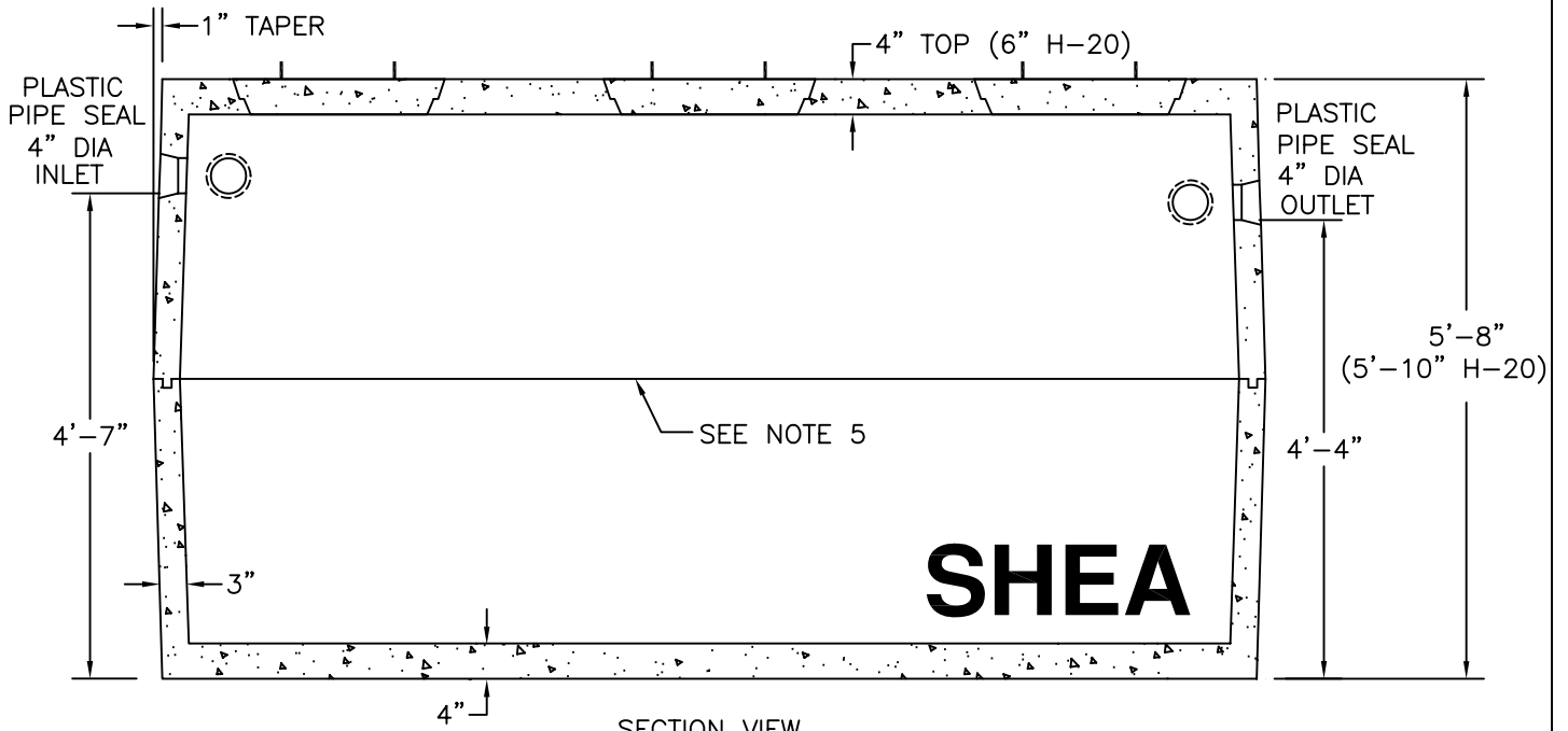
SECTION VIEW
