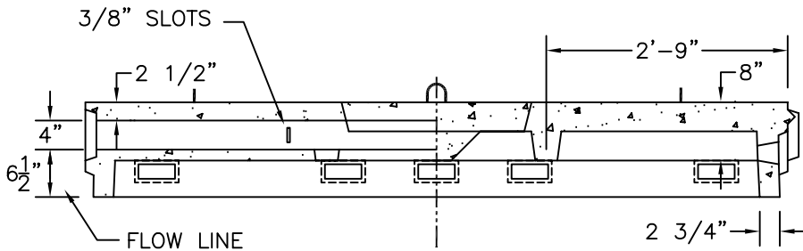
SIDE SECTION VIEW
