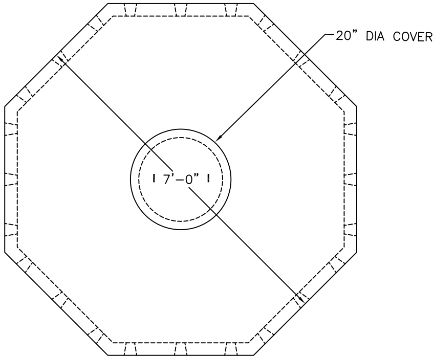
PLAN VIEW
