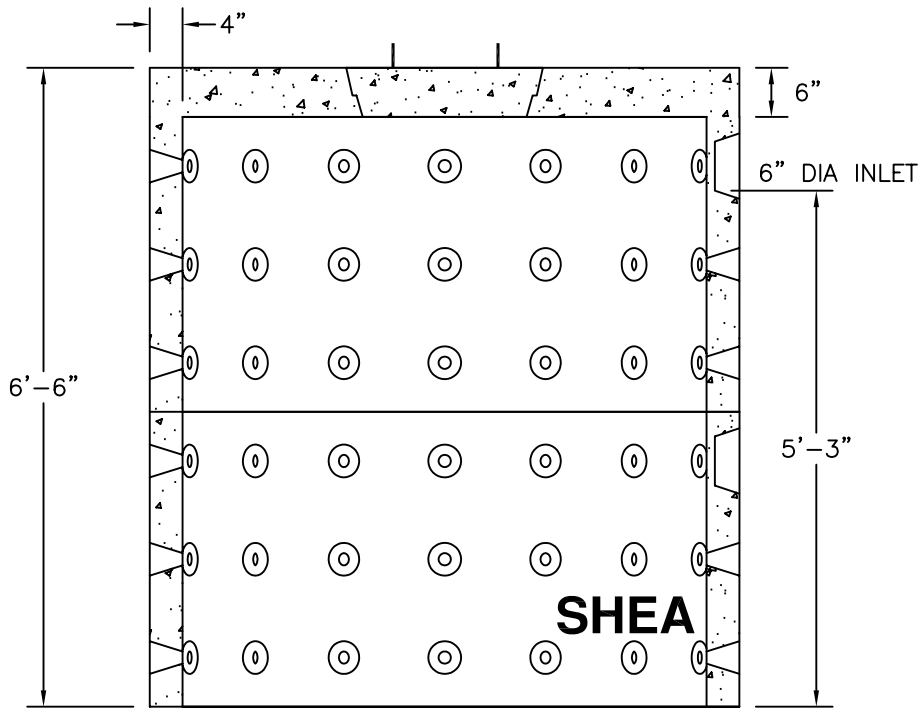
SECTION VIEW
